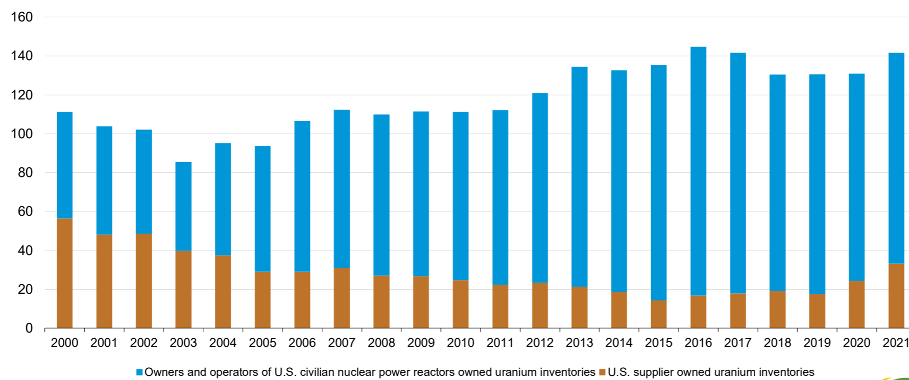
Figure S5. Total commercial uranium inventories of U.S. suppliers and owners and operators of U.S. civilian nuclear power reactors, 2000–2021 million pounds U 3 O 8 equivalent
