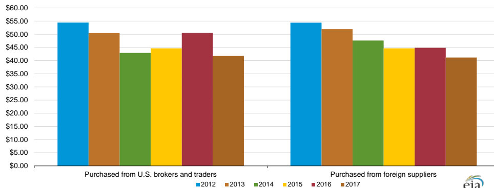
Figure 2. Weighted-average price of uranium purchased by owners and operators of U.S. civilian nuclear power reactors by supplier and delivery year, 2012–17
