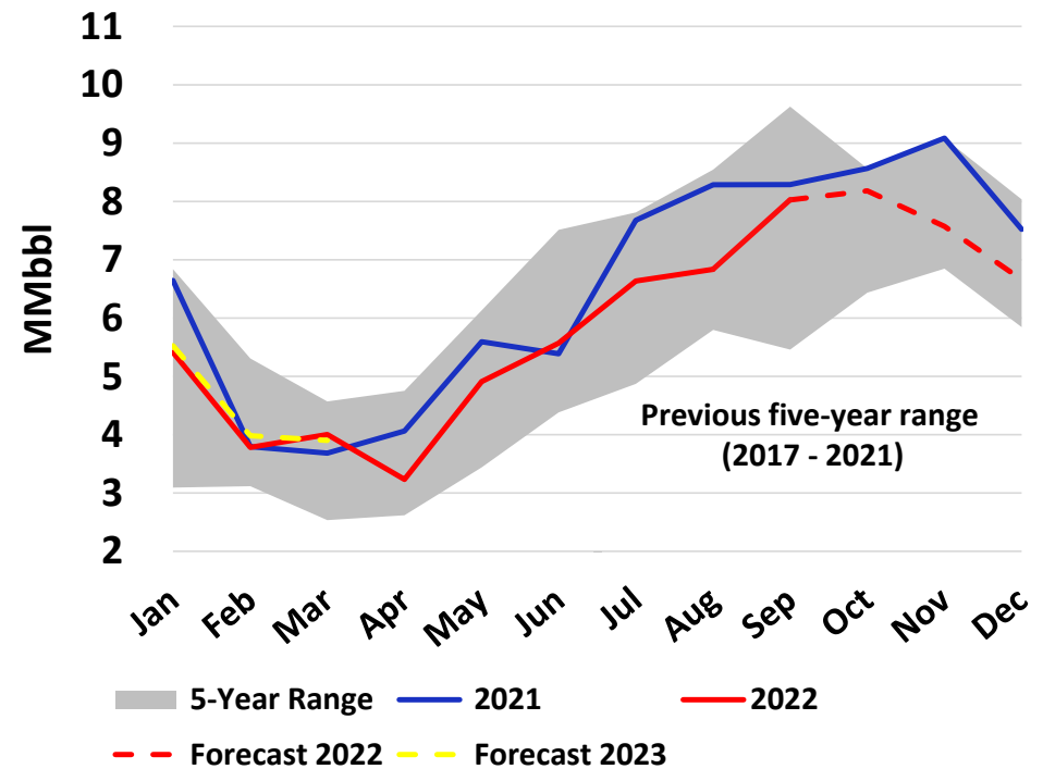
PADD I Monthly Propane Inventory
