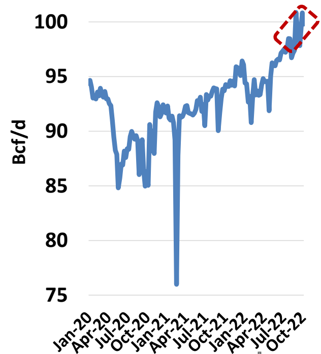
U.S. Lower-48 Gas Production (Dry)
