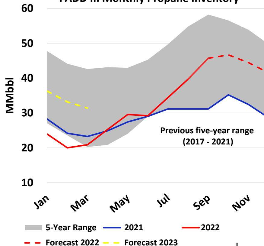
PADD III Monthly Propane Inventory
