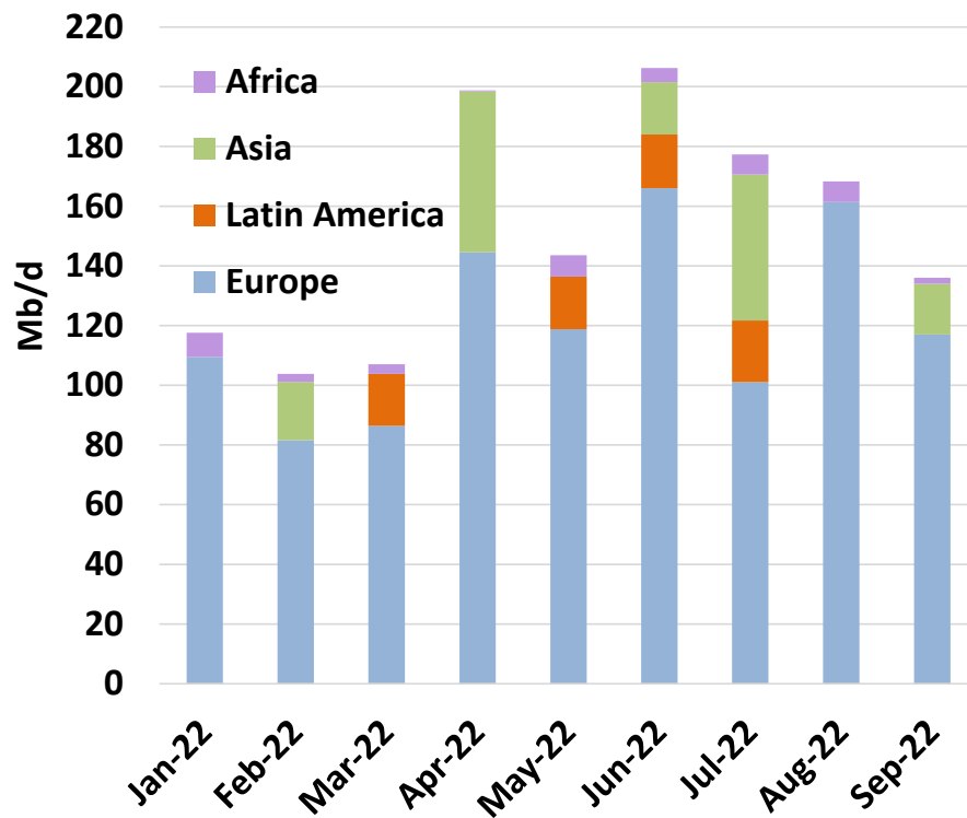
East Coast Propane Exports
