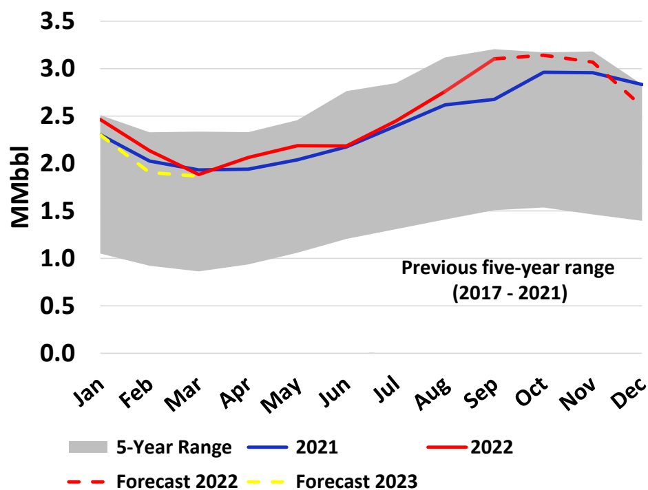
PADD IV Monthly Propane Inventory
