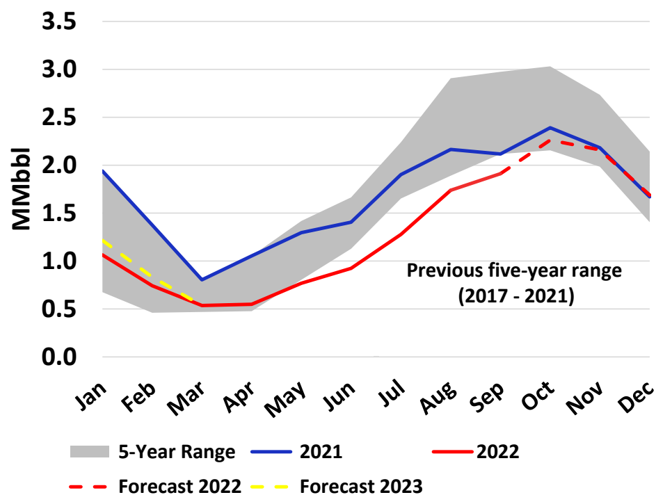
PADD V Monthly Propane Inventory
