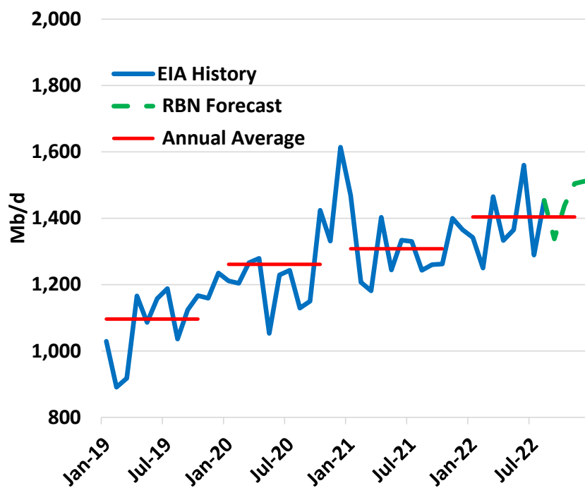
U.S. Waterborne Exports of Propane
