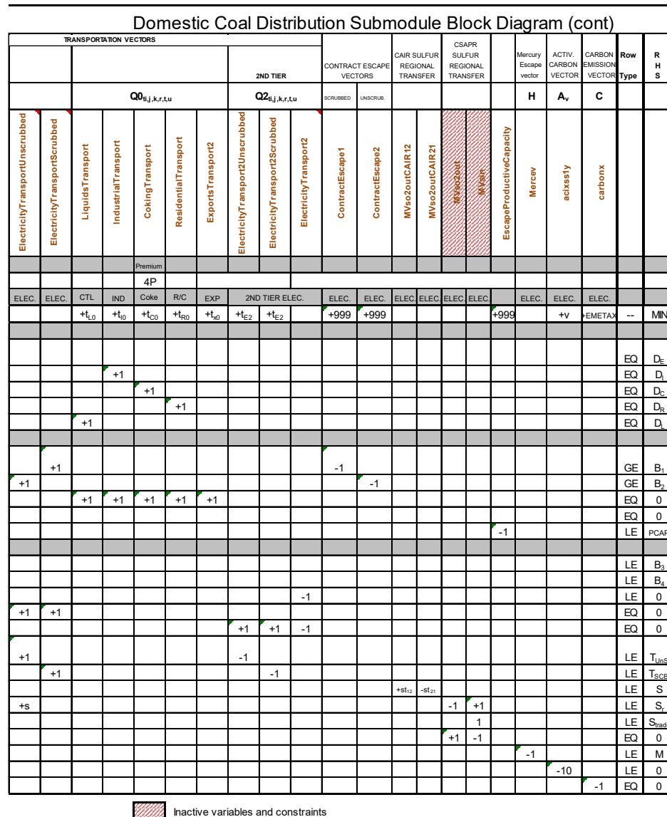
Figure 2.A-2. Linear program structure diagram for the Domestic Coal Distribution Submodule (continued from opposite page)
