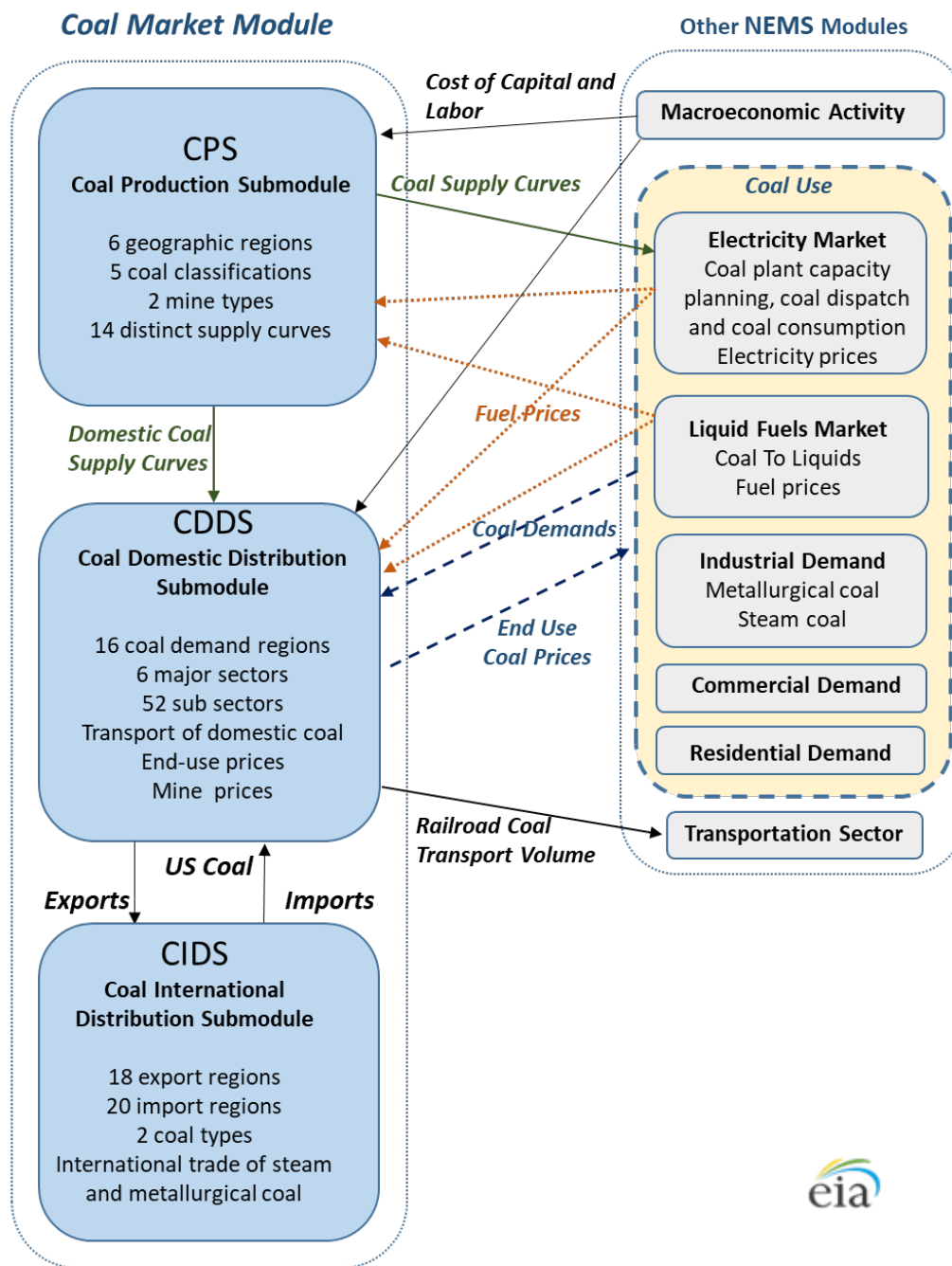
Figure A. Information flow between the Coal Market Module (CMM) and other components of the National Energy Modeling System (NEMS)
