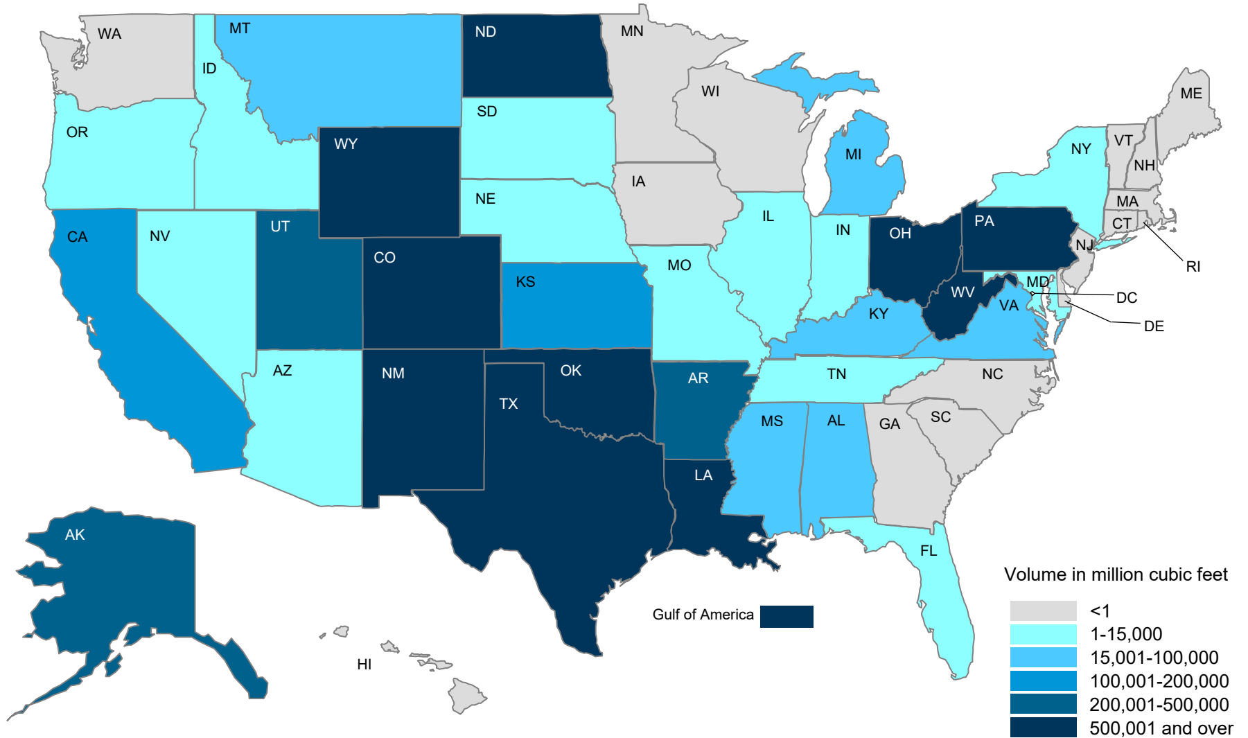
Figure 3. Marketed production of natural gas in the United States and the Gulf of America, 2024 million cubic feet
