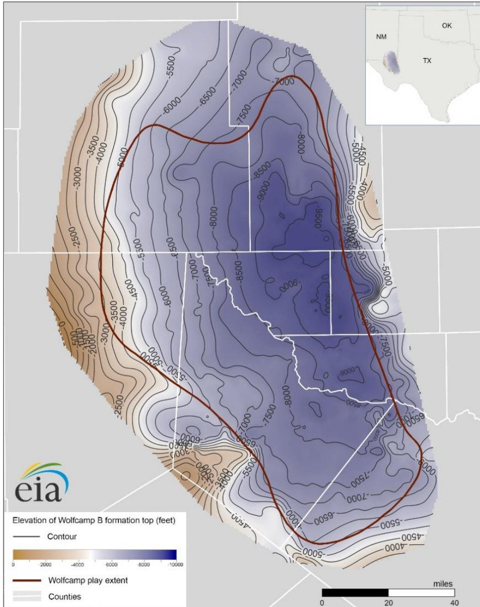
Figure 11. Structure map of Wolfcamp B (Delaware Basin)
