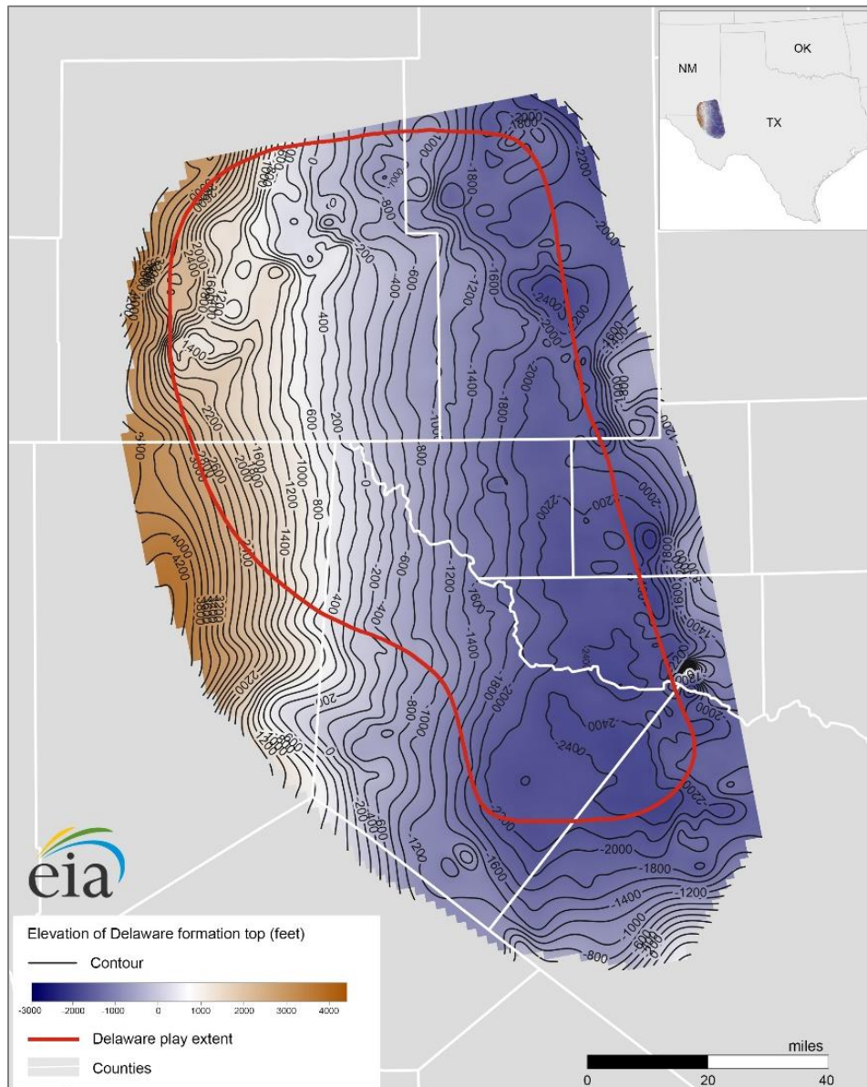
Figure 21. Structure map of the Delaware Mountain Group (Delaware Basin)
