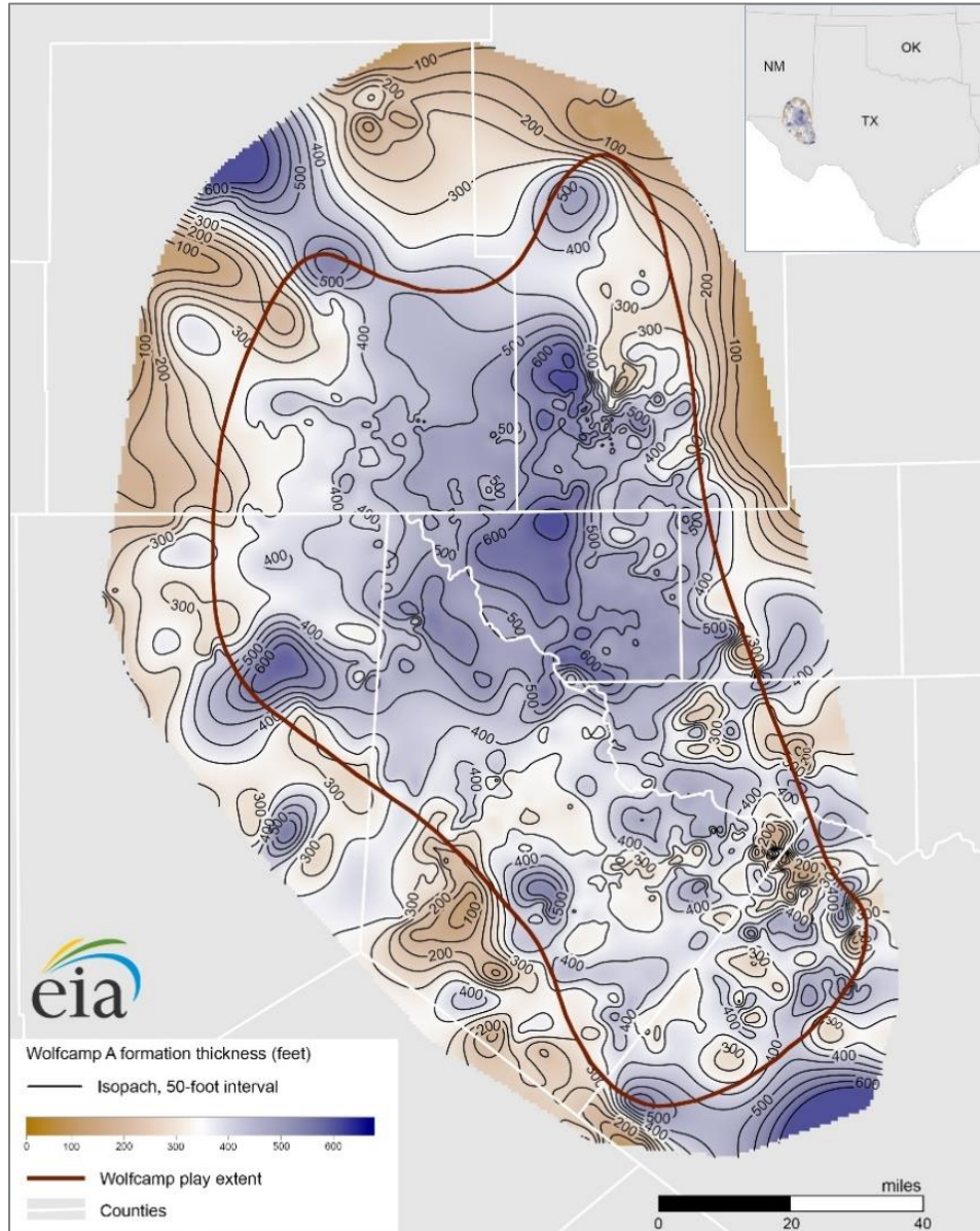
Figure 10. Thickness map of Wolfcamp A (Delaware Basin)
