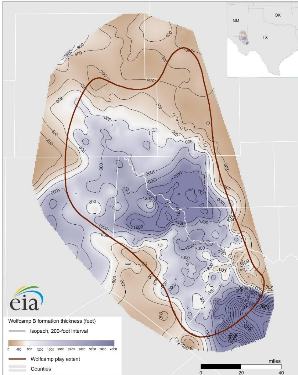
Figure 12. Thickness map of Wolfcamp B (Delaware Basin)
