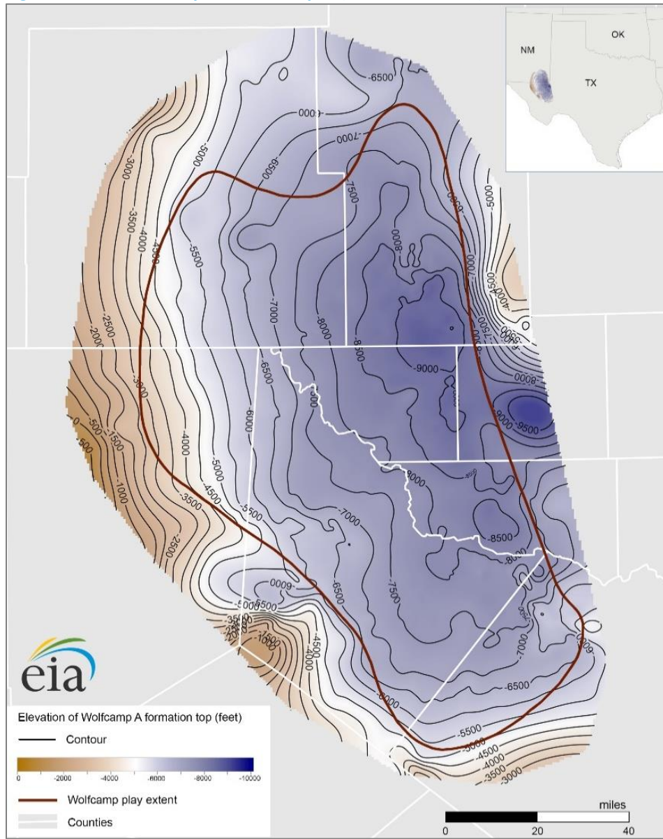
Figure 9. Structure map of Wolfcamp A (Delaware Basin)
