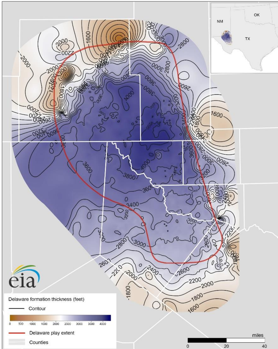
Figure 22. Thickness map of the Delaware Mountain Group (Delaware Basin)
