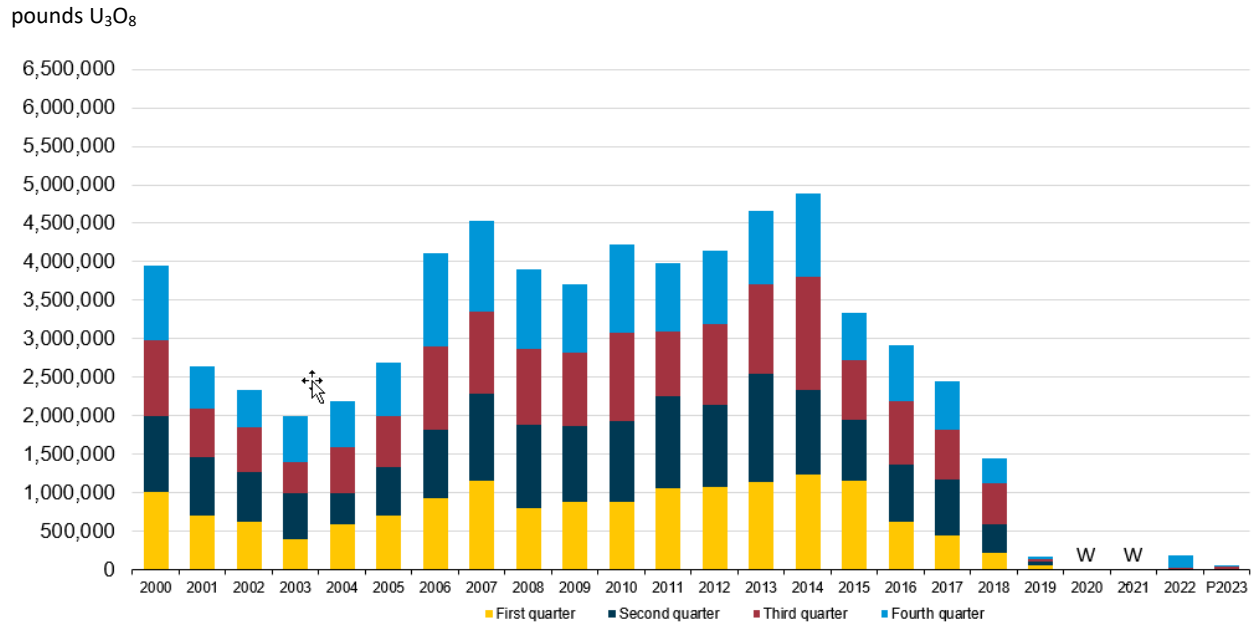
Figure 1. Uranium concentrate production in the United States, 2000 to fourth-quarter 2023
