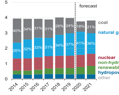
U.S. electricity generation by fuel, all sectors trillion kilowatthours
